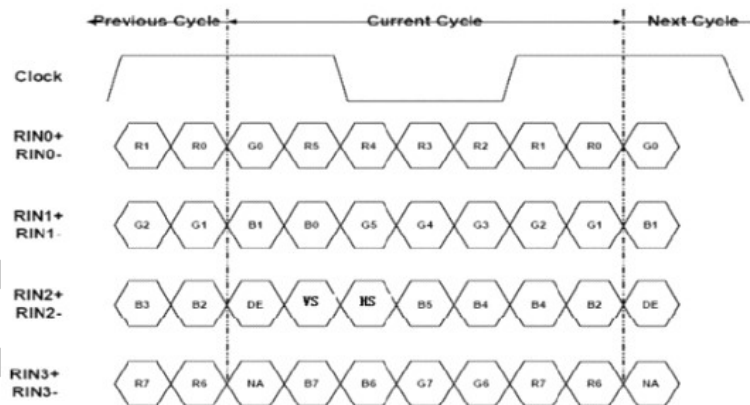
图 5-1 LVDS JEDIA mode and NS mode
